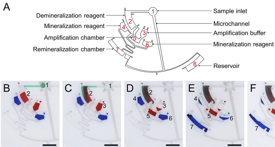
Fig. 4 Operation of the CD microfluidic chip. (A) Structure of the CD microfluidic chip and functional partitions. (B) Original state. Target DNA is mineralized with calcium carbonate nanoparticles in the original sample. (C) The sample in chamber one is driven into chamber two at 350 rpm. Mineralized target DNA is released with reagents for demineralization. (D) The demineralized sample in chamber two and amplification buffer in chamber three are driven into chamber five at 450 rpm. Free target DNA is amplified with RPA reagents. (E) The amplification product in chamber five and mineralization reagents in chambers four and six are driven into chamber seven at 550 rpm. The target DNA is remixed with reagents for mineralization. (F) The remineralized DNA sample in chamber seven is driven back to chamber one under capillary force. The scale bar is 1 cm.
