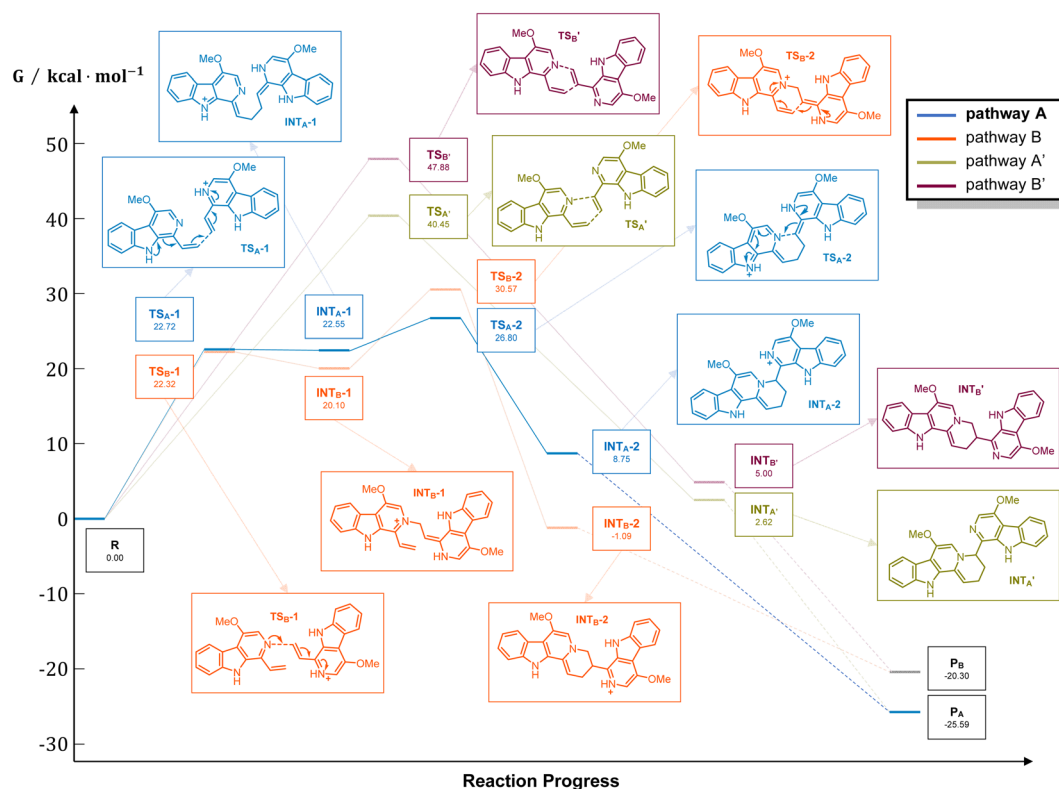
Scheme 3 Energy profile of the aza-[4 + 2] cycloaddition. For pathways A and B, R = 1 × dehydrocraenatine ( 10a ) and 1 × protonated dehydrocraenatine; for pathways A' and B', R = 2 × dehydrocraenatine. P A = picrasidine G ( 1 ), P B = isopicrasidine G. Calculation at WB97XD/6-311++G(2d,p)//WB97XD/6-31G(d) at 403.15 K. Gibbs free energies ( \Delta G ) are in kcal mol −1 .
