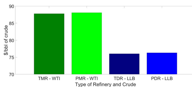
Fig. 8 Cost of energy incorporated into the cost of oil per barrel. With the cost of WTI at $85 and the cost of the Llyod Minster blend at $72, the energy cost is a small percent increase in the total cost per barrel. The TMR energy cost adds $2.79 while the PMR adds $3.08 resulting in a net increase cost of only 0.33%. Similarly, for the TDR, the energy cost adds $4.02 while the PDR adds $4.31 resulting in a net increase cost of only 0.38%. All $ values are in USD.
