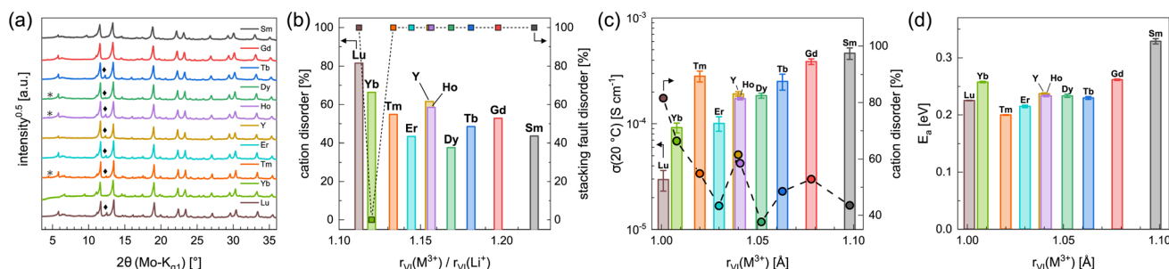
Fig. 5 (a) PXRD diffraction patterns and (b) degrees of intra-layer cation disorder and stacking fault disorder obtained from Rietveld refinements of the different Li 3 MI 6 . Asterisks and diamonds correspond to impurities of MOI and MI 3 , respectively. In (c) ionic conductivities at 20 °C with intra-layer cation disorder and in (d) activation energies for ion diffusion obtained from EIS are shown as a function of the ionic radii 43–45 of the rare earth metal cations.
