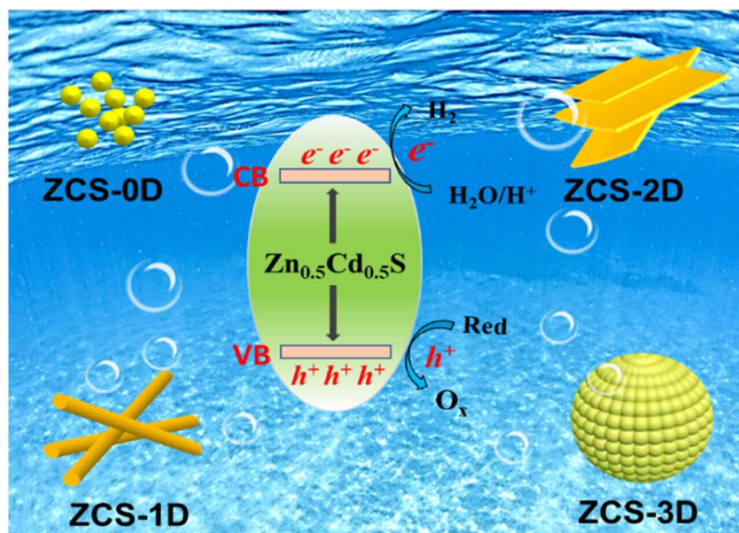
Fig. 10 Photocatalytic mechanism of \text{H}_2 production on ZCS materials with different morphologies.
