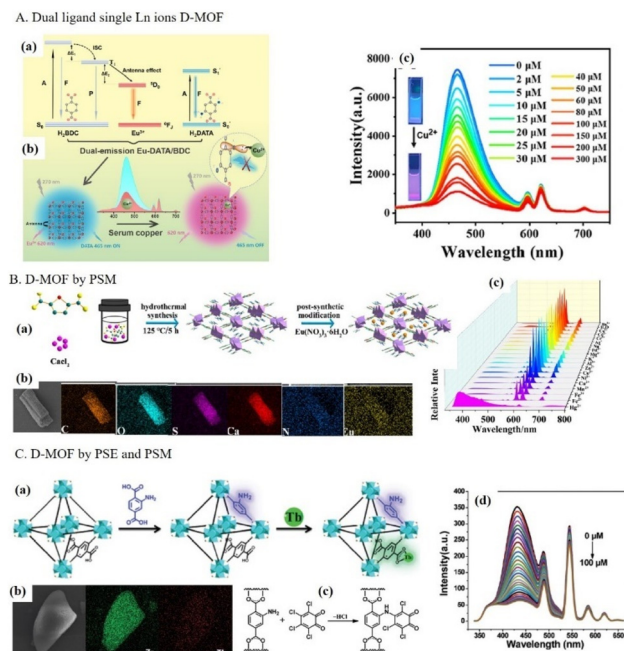
Fig. 13 (A) The design principle and preparation of \text{Eu}-\text{DATA}/\text{BDC} , where \text{H}_2\text{BDC} sensitizes \text{Eu}^{3+} ions to realize the antenna effect emission and \text{DATA} maintains its own emission and identifies \text{Cu}^{2+} ions, and the fluorescence spectra of \text{Eu}-\text{DATA}/\text{BDC} in aqueous solutions with \text{Cu}^{2+} ions at different concentrations. Reproduced with permission from ref. 199. Copyright 2022, Elsevier. (B) \text{Eu}-\text{Ca}-\text{MOF} prepared by PSM. (a) The synthesis of \text{Eu}-\text{Ca}-\text{MOF} . (b) The EDX element mapping diagram of \text{Eu}-\text{Ca}-\text{MOFs} and (c) the emission spectra of \text{Eu}-\text{Ca}-\text{MOFs} after treatment with different metal ions. Reproduced with permission from ref. 212. Copyright 2023, Elsevier. (C) The construction of D-MOFs by PSE. (a and b) The synthesis procedure, SEM image, and SEM-EDX elemental mapping of \text{Tb}@\text{UiO}-66-(\text{COOH})_2\text{NH}_2 . (c) The mechanism of capturing o-TCBQ by \text{atp}^{2-} ligand. (d) The photoluminescence spectra of \text{Tb}@\text{UiO}-66-(\text{COOH})_2\text{NH}_2-40 at different concentrations of o-TCBQ. Reproduced with permission from ref. 220. Copyright 2016, the American Chemical Society.
