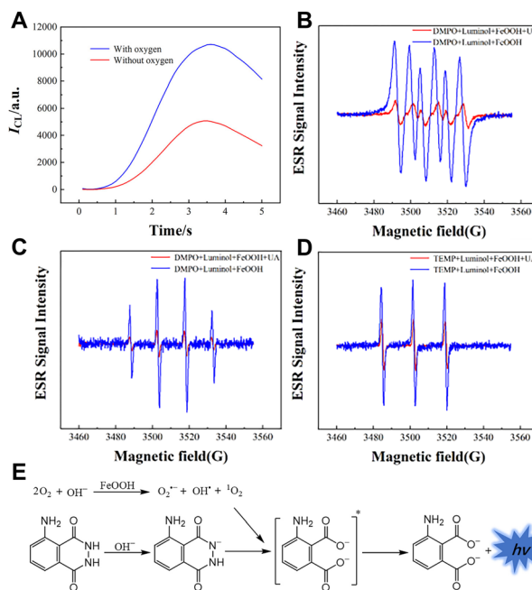
Fig. 12 (A) CL kinetic curves of the luminol/FeOOH system in the absence and presence of oxygen. ESR spectra of adducts. (B) DMPO- \text{O}_2^{\bullet-} (C) DMPO- \text{OH}^{\bullet} and (D) TEMP- ^1\text{O}_2 in the luminol/FeOOH CL system. (E) Mechanism of the luminol/FeOOH CL system. [Luminol]: 100 \mu\text{M} ; [FeOOH]: 25 \mu\text{g mL}^{-1} ; [UA]: 5 \mu\text{M} ; [pH]: 10.0. Reprinted with permission from ref. 63, Copyright 2023 American Chemical Society.
