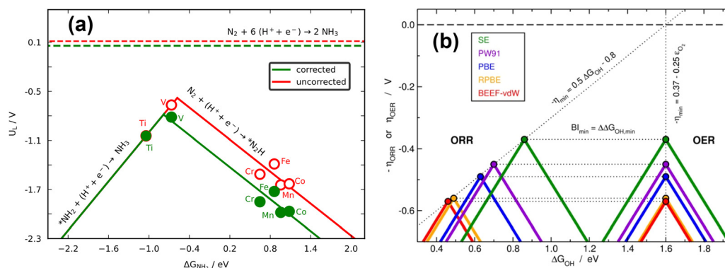
Fig. 17 (a) Volcano plot for electrochemical ammonia synthesis on different metaloporphyrins. In red: PBE results with no gas-phase corrections. In green: corrected PBE results. The dashed lines represent the equilibrium potentials. Reproduced from ref. 29, licensed under CC BY 4.0 ( https://creativecommons.org/licenses/by/4.0/ ). (b) Volcanoes obtained with four GGAs for the OER and ORR. After accounting for all the gas-phase errors, a single semiempirical volcano (in green, SE) is obtained for each reaction. BI: bifunctional index for the ORR/OER redox performance. Reproduced from ref. 42, licensed under CC BY-NC-ND 4.0 ( https://creativecommons.org/licenses/by-nc-nd/4.0/ ).
