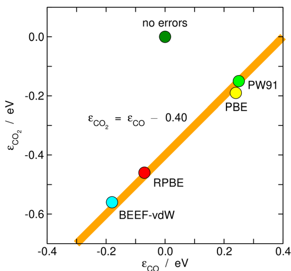
Fig. 7 Correlation between the gas-phase errors in CO and CO 2 for various xc-correlation functionals. The hypothetical perfect agreement between DFT and experimental values is marked in dark green.
