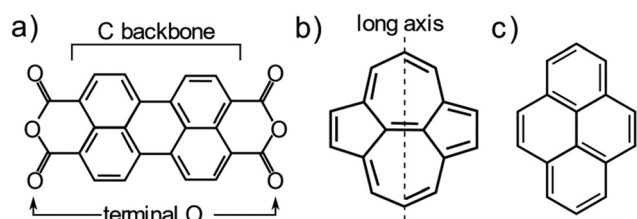
Fig. 1 Molecular structure of (a) PTCDA, (b) azulopyrene and (c) pyrene.
