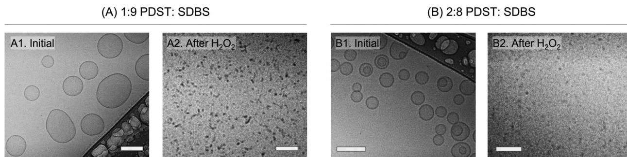
Fig. 4 Cryo-TEM images confirming the ROS-induced VMT. The images are of (A) 1:9 and (B) 2:8 PDST:SDBS samples before and after the addition of 15% \text{H}_2\text{O}_2 . Images A1 and B1 show that the initial samples mostly contain unilamellar vesicles with sizes of 100–200 nm. Images A2 and B2 show no vesicles and instead the presence of small spherical or cylindrical micelles ( \sim 5 –10 nm). Thus, the images confirm that ROS from \text{H}_2\text{O}_2 induce a VMT. Scale bars: 100 nm.
