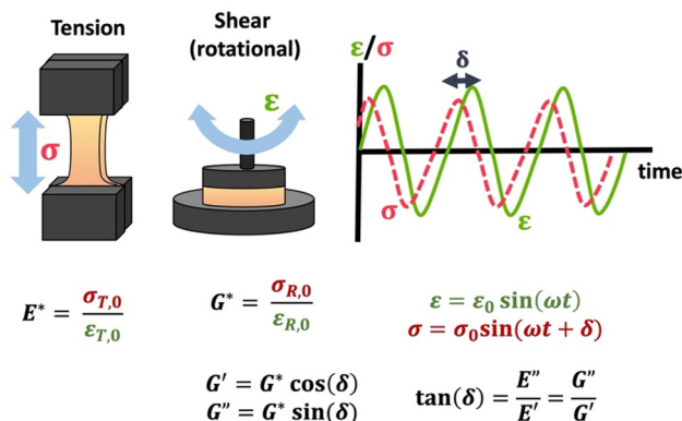
Scheme 12 Schematic of tensile DMA and SAOR, including \sigma response to sinusoidally applied \varepsilon , and the complex moduli E^*/G^* and the storage ( E'/G' ) and loss ( E''/G'' ) moduli. Note that \sigma_{T,0} , \varepsilon_{T,0} , \sigma_{R,0} , and \varepsilon_{R,0} are given in Table 1.
