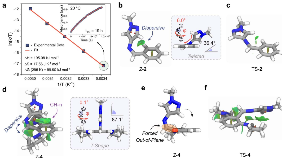
Fig. 5 (a) Eyring plot of the longest-lived Z-AIP, 4 . (inset) Rate of thermal reversion of the Z-to-E isomer at 20 °C. (b) Geometry-optimized Z-2 highlighting green NCI surfaces between the pyrazole and phenyl rings. (inset) Display of the twisted geometry. (c) Geometry-optimized TS-2 with NCI surfaces displayed. (d) Geometry-optimized Z-4 showing large NCI interactions between the imine and the ortho -pyrrolidine units, as well as CH- \pi interactions between the CH of the pyrazole and the phenyl ring. (inset) View showing the T-Shape conformation. (e) Alternate view of Z-4; the pyrrolidine projecting out of the page is depicted as a red stub for clarity. (f) Geometry-optimized structure of TS-4 with NCI surfaces displayed.
