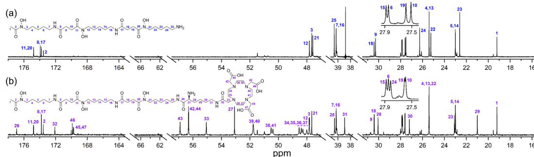
Fig. 2 { 1 H}- 13 C NMR spectra from solutions (D 2 O) of (a) 1 or (b) 3a .
