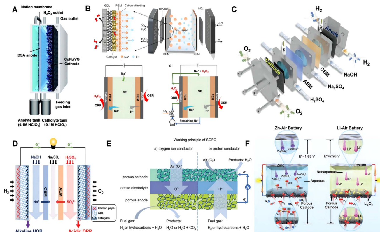
Fig. 15 (A) Schematic of the flow cell setup utilizing Co/N 4 /VG as the cathode. Reproduced from ref. 254 with permission. Copyright 2022, Royal Society of Chemistry. (B) Schematic illustration of reducing \text{O}_2 to \text{H}_2\text{O}_2 in our SE cell with a double-PEM configuration. Reproduced from ref. 255 with permission. Copyright 2022, Nature Publishing Group. (C) Schematic illustration of the CF-FC system with 2.0 M \text{H}_2\text{SO}_4 and 4.0 M \text{NaOH} as the catholyte and anolyte, respectively. (D) Schematic illustration of the CF-FC consisting of an acidic ORR chamber (0.5 M \text{H}_2\text{SO}_4 ). Reproduced from ref. 17 with permission. Copyright 2024, Wiley-VCH GmbH. (E) Working principle of the SOFC with an oxygen-ion conductor electrolyte (SOFC). Reproduced from ref. 256 with permission. Copyright 2022, Wiley-VCH GmbH. (F) Reproduced from ref. 257 with permission. Copyright 2024, Wiley-VCH GmbH.
