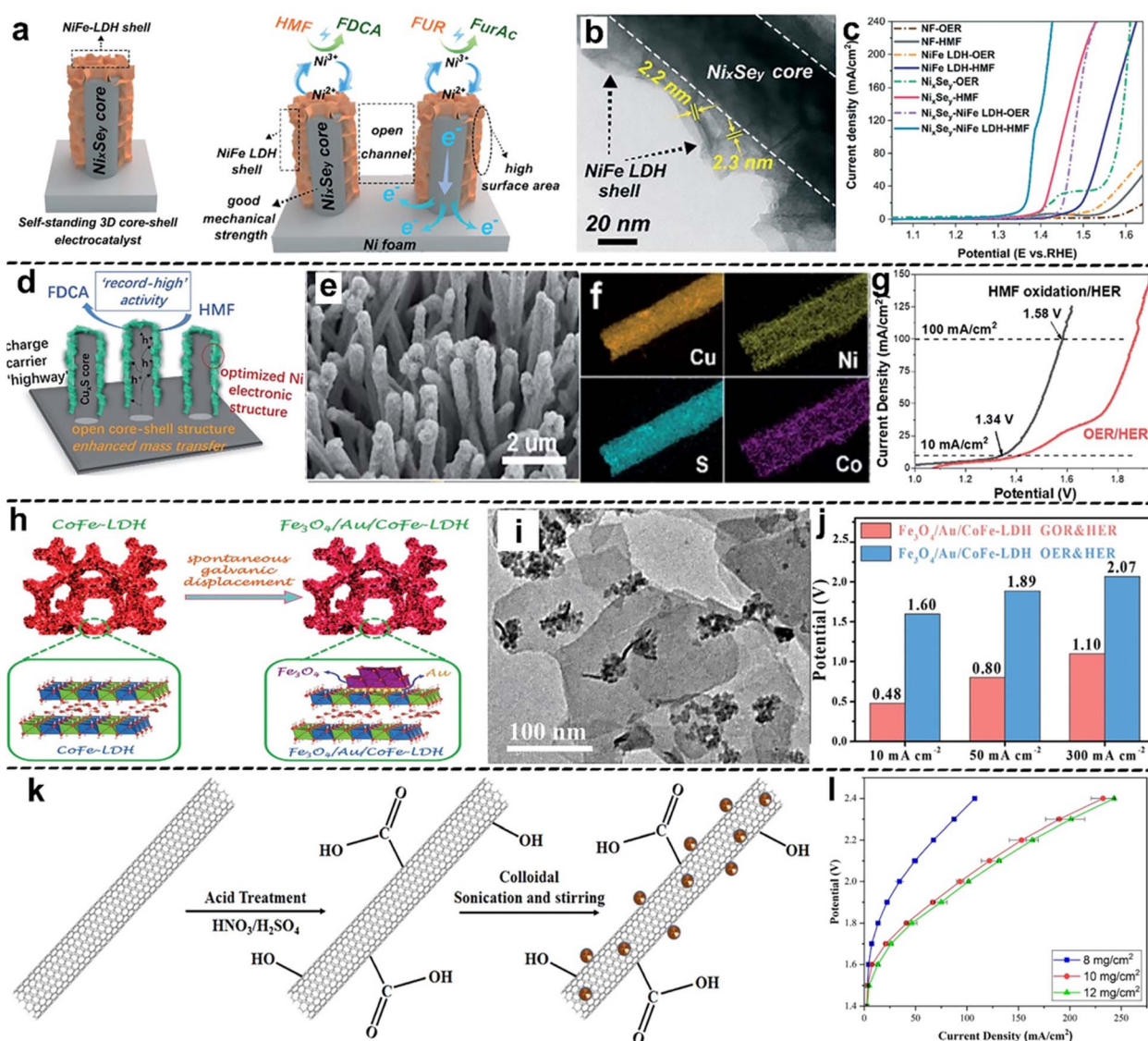
Fig. 5 Selected examples for the Construction of heterostructures subsection: (a) the schematic structure and the mechanism proposed for the electrooxidation of HMF and furfural (FUR) on the Ni x Se y -NiFe LDH@NF electrode, (b) TEM images of the Ni x Se y -NiFe LDH core-shell structure, (c) LSV curves of NF, NiFe LDH@NF, Ni x Se y @NF and Ni x Se y -NiFe LDH@NF (these figures have been reproduced from ref. 87 with permission from Royal Society of Chemistry, copyright 2022), (d) schematic illustration, (e) SEM image and (f) elemental mapping of Cu x S@Ni 0.75 Co 0.25 O x H y /CF, (g) LSV curves for the OER/HER and HMFOR/HER over the bifunctional Cu x S@Ni 0.75 Co 0.25 O x H y /CF electrode (these figures have been reproduced from ref. 88 with permission from Royal Society of Chemistry, copyright 2020), (h) synthetic route and (i) TEM image of CoFe-LDH and Fe 3 O 4 /Au/CoFe-LDH, (j) cell potential of the GOR/HER and OER/HER at different current densities with iR -compensation (these figures have been reproduced from ref. 89 with permission from Wiley, copyright 2021), (k) synthetic approach for PbO 2 /MWNTs for the LOR, and (l) LSV curve from different PbO 2 /MWNT catalyst loading samples (these figures have been reproduced from ref. 90 with permission from IOP Publishing, copyright 2019).
