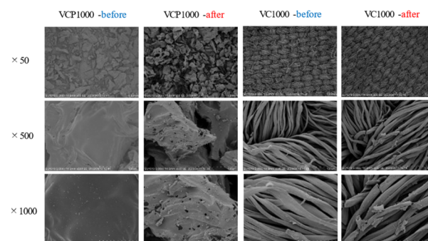
Fig. 7 The SEM images of VCP1000 and VC1000 before and after adsorption. Initial concentration, 100 mg L -1 ; sample volume, 50 mL; adsorbent, 0.02 g; temperature, 25 °C; contact time, 24 h, 100 rpm.
