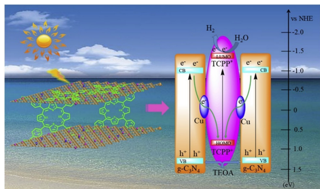
Fig. 38 Scheme of the TCPP-Cu-g-C 3 N 4 composite and illustration of the separation and transfer of photo-produced charges promoted by this photocatalyst. Reproduced from ref. 164. Copyright 2019 Elsevier.
