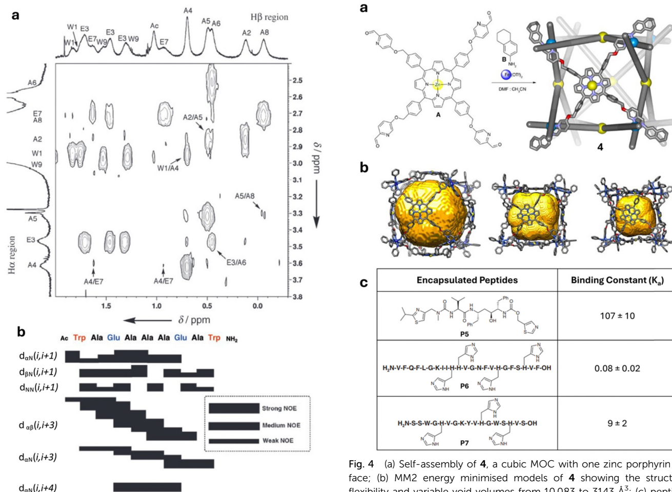
Fig. 3 (a) Selected NOESY spectrum for the assignment of bound peptide (600 MHz, \text{H}_2\text{O}/\text{D}_2\text{O} = 9/1 , 27 °C, 100 mM phosphate buffer, pH 6.8), [2] = 10 mM, [peptide] = 2.5 mM. Proton resonances labelled with single letter amino acid code and residue number corresponding to peptide in Fig. 2a; (b) NOE correlations for peptide 2 . Reproduced with permission from ref. 16.
