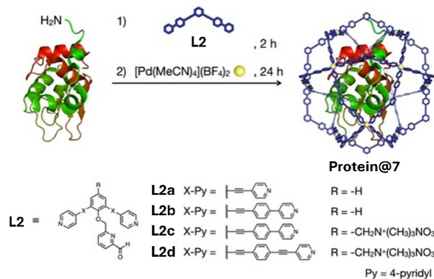
Fig. 5 Encapsulation of a protein within a M 12 L 24 MOC (7) and the range of linkers (L 2 a–d) employed to generate isostructural cages with a range of internal void cavities. Reproduced with permission from ref. 22.
