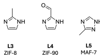
Fig. 6 Imidazole linkers most commonly employed in enzyme@MOF in situ synthesis procedures including coprecipitation and biomimetic crystallisation approaches. ZIF-8 incorporates L 3 , ZIF-90 incorporates L 4 and MAF-7 incorporates L 5 .
