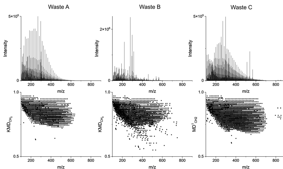
Fig. 7 Upper panel: HRMS spectra of three waste plastic samples obtained from integrated pyro-(−)DART thermograms. Lower panel: \text{CH}_2 -based Kendrick mass defect ( \text{KMD}_{\text{CH}_2} ) plots. Samples are Waste A (left), Waste B (middle), and Waste C (right).
