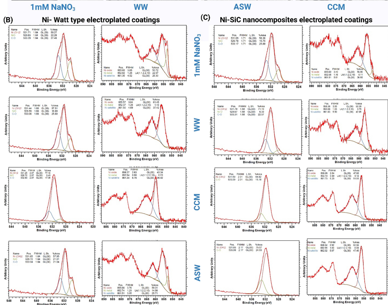
Fig. 3 Characterisation of Ni Watt type and Ni-SiC nanocomposite electroplated coating post aging in various media. (A) TEM analysis of Ni-SiC electroplated aging in artificial sea water (ASW), wastewater (WW), cell culture media (CCM), and 1 mM NaNO 3 . XPS analysis of Ni-Watts type coatings (B) and Ni-SiC (C) nanocomposite coatings in various simulated media showing transformation of Ni in various media. The chemical composition and respective peaks for Ni and O are shown in the graphs.
