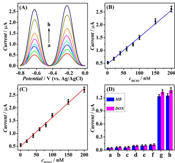
Fig. 6 (A) DPV curves to HClO and H 2 O 2 with different concentrations (from (a) to (h): 1, 20, 40, 60, 80, 100, 150, and 200 nM). The linear fit of (B) I_{\text{DOX}} versus c_{\text{HClO}} and (C) I_{\text{MB}} versus c_{\text{H}_2\text{O}_2} . (D) Selectivity of the sensing system for HClO (80 nM) and H 2 O 2 (80 nM) against other interferents of 800 nM: (a) blank, (b) NaNO 2 , (c) UA, (d) AA, (e) NaNO 3 , (f) GSH, (g) HClO and H 2 O 2 , and (h) the mixture of HClO, H 2 O 2 , and interferents. Error bar: SD and n = 3 .
