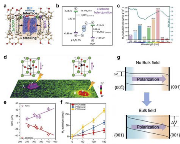
Fig. 10 (a) Intramolecular built-in electric field to enhance photo-generated charge separation. Reproduced with permission from ref. 127 Copyright 2022 Wiley. (b) Construction of Z-scheme charge transfer mechanism. Reproduced with permission from ref. 128 Copyright 2021 Wiley. (c) Overlay of wavelength-dependent hydrogen evolution and UV-vis absorption. Reproduced with permission from ref. 129 Copyright 2021 Wiley. (d) Image of ferroelectric field visualization. (e) Statistical SPV data of \text{PTO}_3 . (f) Photocatalytic hydrogen evolution activity of three PTO samples with cocatalysts. (g) Schematic representation of ferroelectric field affecting the energy band structure. Reproduced with permission from ref. 130 Copyright 2020 Wiley.
