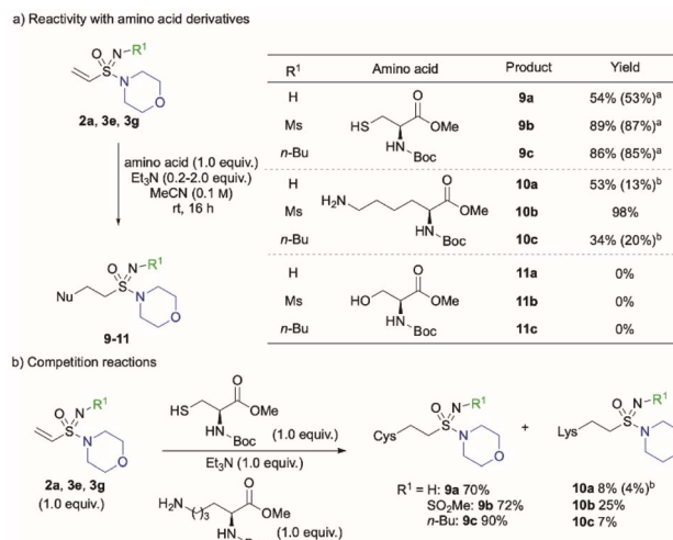
Scheme 3 Conjugate addition reaction of vinyl sulfonimidamides 2–3 with amino acid derivatives. Reaction conditions: cysteine: Boc-(L)-Cys-OMe (1.0 equiv.), Et 3 N (1.0 equiv.), MeCN, rt, 16 h; lysine: Boc-(L)-Lys-OMe-HCl (1.0 equiv.), Et 3 N (2.0 equiv.), MeCN, rt, 16 h; serine: Boc-(L)-Ser-OMe (1.0 equiv.), Et 3 N (1.0 equiv.), MeCN, rt, 16 h. Isolated yields reported. a Et 3 N (0.2 equiv.) was used; b yield for double addition product.
