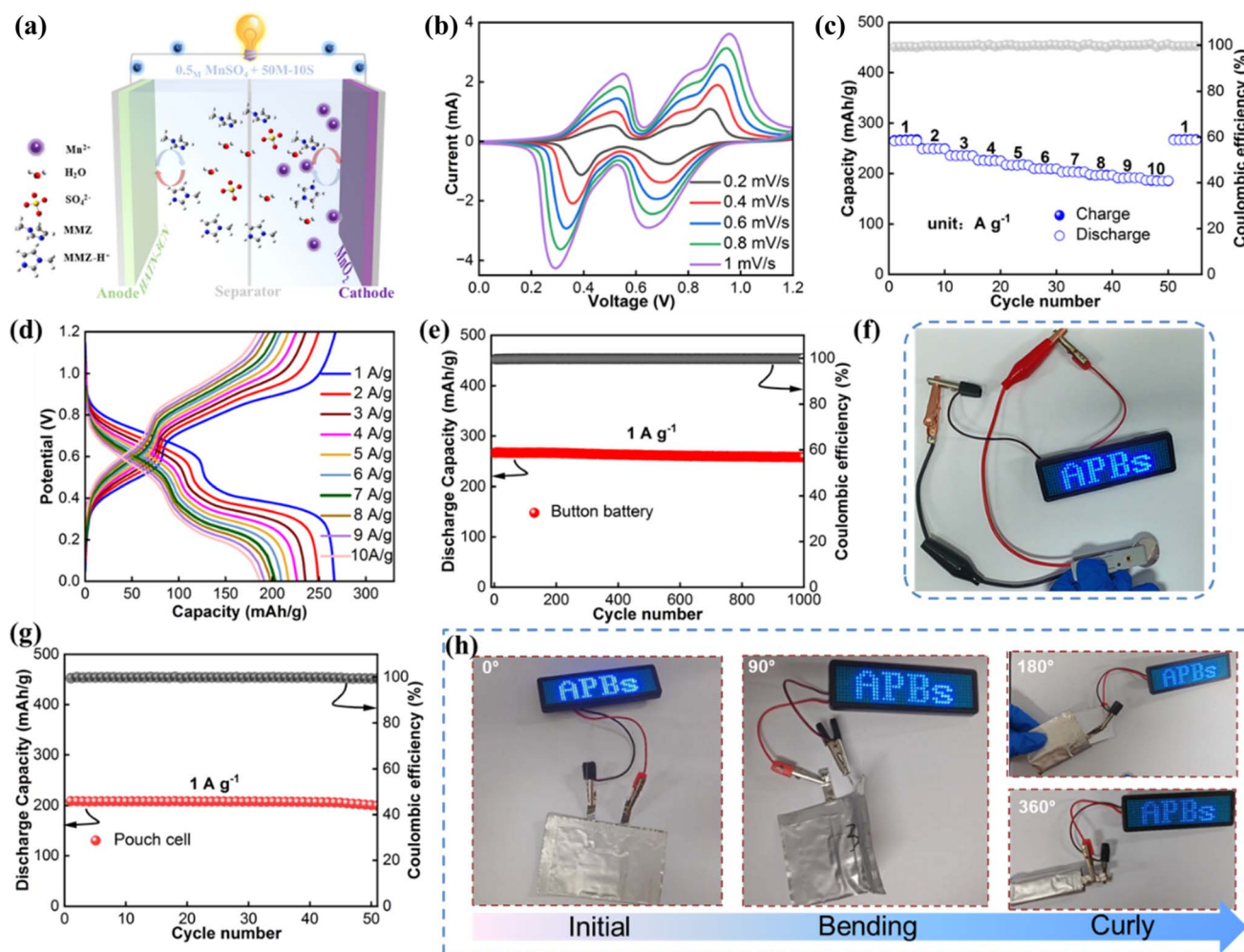
Fig. 6 Electrochemical performance of the HATN-3CN// MnO_2 full battery. (a) Schematic illustration of the full battery. (b) CV curves at different scan rates from 0.2 to 1 mV s^{-1} , (c) rate performance, (d) charge–discharge curves, (e) cycling performance at 1 A g^{-1} and (f) optical image of an LED screen powered by a button-type battery. (g) Cycling performance at 1 A g^{-1} and (h) optical image of an LED screen powered by the pouch cell.
