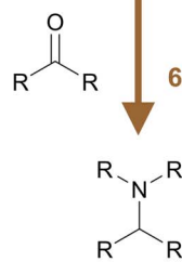
Fig. 6 Common reactions performed in methylene chloride (numbered 1 to 8). Numbers are the popularity ranking of each reaction according to SciFinder for the period between January 2020 and March 2025. The schemes represent generic versions of the most common transformations found within each category.
