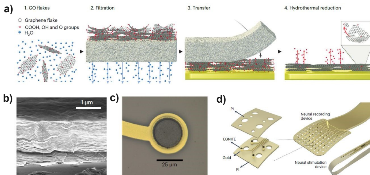
Figure 10 Preparation and transfer of rGO thin films via EGNITE process (a). SEM image of the film cross-section showing dense package of rGO flakes (b). Optical image of the finalized rGO coating (c) and illustration of the final in vivo devices (d). Reproduced from reference 75 , with permission from Nature, Copyright 2024.
