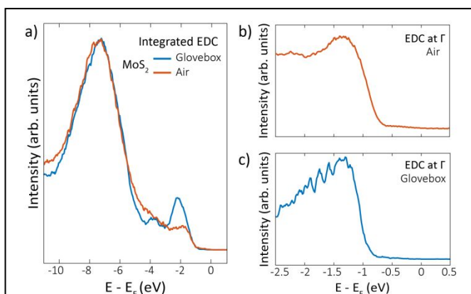
Fig. 2: Valence band for the air (red) and glove-box (blue) sample, taken in normal emission with 95 eV photon energy. (a) EDCs angle-integrated \sim 0.3 \text{ \AA}^{-1} around the \Gamma point of the SBZ. (b and c): angle-resolved EDC's taken at normal emission at \Gamma ( 0.07 \text{ \AA}^{-1} acceptance).
