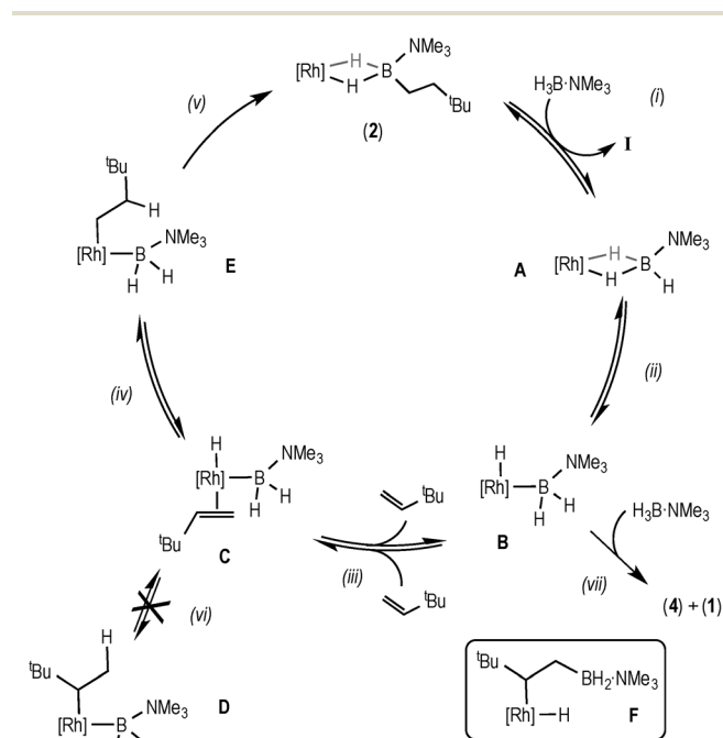
Scheme 6 Proposed mechanism for the catalytic hydroboration using data from the early phase of catalysis. [\text{Rh}] = [\text{Rh}(\text{xantphos})]^+ .
