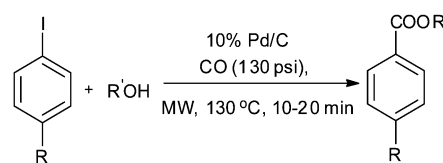
Scheme 39 Reagents and conditions: aryl iodide (0.50 mmol), alcohol (0.50 mmol), DMF (1 mL), DBU (224 \mu\text{L} , 1.50 mmol), Pd/C 10% (10 mg, 0.01 mmol), CO (130 psi), temp. MW, 130^\circ\text{C} at 150 W, time 20 min.
