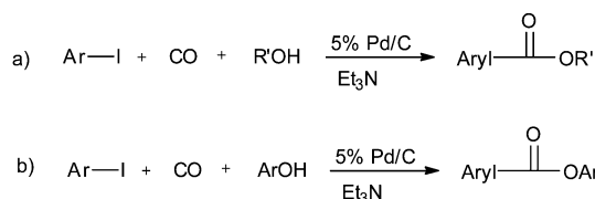
Scheme 38 Reagents and conditions: (a) iodobenzene (2.5 mmol), 5% Pd/C (5 mg), \text{Et}_3\text{N} (7.2 mmol), alcohol (4 mL), CO (0.5 MPa), temp. 130^\circ\text{C} , time 2 h; (b) iodobenzene (2.5 mmol), ArOH (3 mmol), 5% Pd/C (30 mg), \text{Et}_3\text{N} (7.2 mmol), toluene (4 mL), CO (2.0 MPa), temp. 130^\circ\text{C} , time 8 h.
