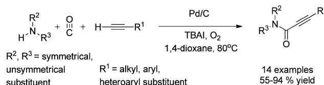
Scheme 42 Reagents and conditions: alk-1-yne (1 mmol), secondary amine (1.5 mmol), 10% Pd/C (8 mol%), CO/O 2 pressure (5/1 atm), TBAI (0.90 mmol), 1,4-dioxane (10 mL), temperature 80^\circ\text{C} , time 14 h.
