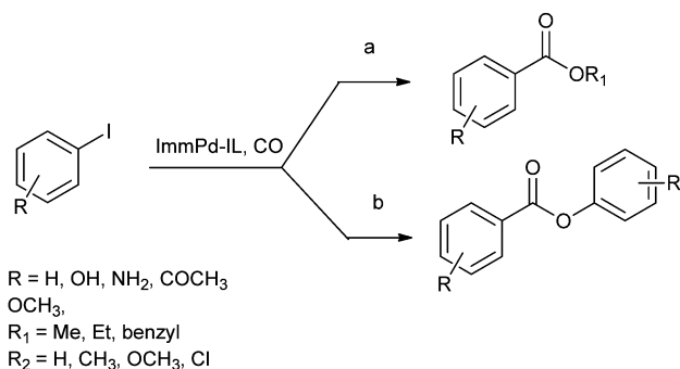
Scheme 41 Reagents and conditions: (a) aryl iodide (1 mmol), alcohol (5 mL), ImmPd-IL (2 mol%), \text{Et}_3\text{N} (3 mmol), CO pressure (0.5 MPa), temp. 80^\circ\text{C} , time 3 h; (b) aryl iodide (1 mmol), phenol (2 mmol), ImmPd-IL (2 mol%), \text{Et}_3\text{N} (3 mmol), toluene (10 mL), CO pressure (1 MPa), temp. 100^\circ\text{C} , time 8 h.
