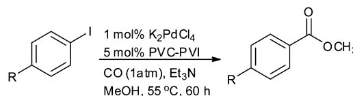
Scheme 40 Reagents and conditions: aryl iodide (0.2 mmol), \text{Et}_3\text{N} (0.4 mmol), \text{K}_2\text{PdCl}_4 (1 mol%), PVI-PVC (70 : 30) (5 mol%), methanol (2 mL), temp. 55^\circ\text{C} , time 60 h.
