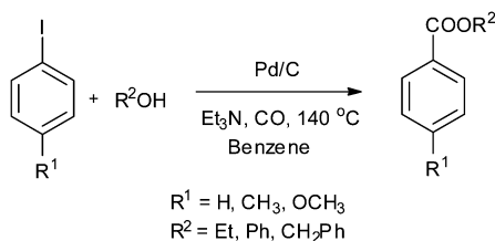
Scheme 37 Reagents and conditions: aryl iodide (2.5 mmol), alcohol (2.5–3.0 mmol), \text{Et}_3\text{N} (3 mmol), 5% Pd/C (50 mg), benzene (5 mL), carbon monoxide (1 MPa), temp. 140^\circ\text{C} , time 6 h.
