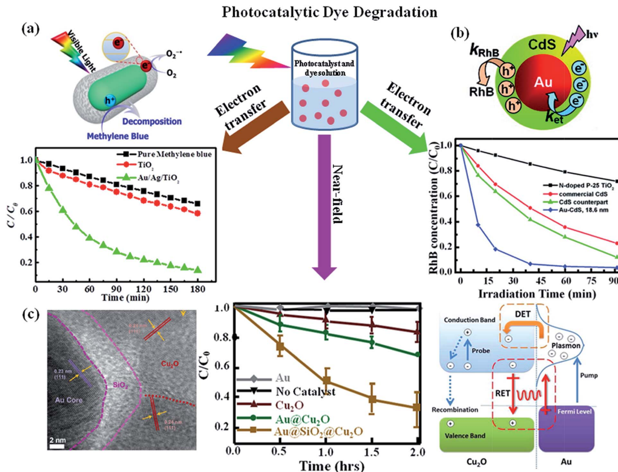
Fig. 9 Photocatalytic dye degradation: (a) photocatalytic degradation of MB under visible light irradiation in the absence and presence of photocatalysts (P25- \text{TiO}_2 , \text{Au}/\text{TiO}_2 or \text{Au}/\text{Ag}/\text{TiO}_2 core-shell NPs) and the schematic representation for the mechanism of photocatalytic degradation of dyes upon visible light excitation of \text{Au}/\text{TiO}_2 NRs. (b) Photocatalytic degradation of RhB in the presence of \text{Au}/\text{CdS} , \text{CdS} and P25- \text{TiO}_2 . The data shows that \text{Au}/\text{CdS} NPs exhibit higher catalytic activity and the proposed mechanism to explain the plasmonic metal enhancement is shown in schematic representation. (c) TEM image of \text{Au}/\text{SiO}_2/\text{Cu}_2\text{O} NP section, visible-light photodegradation of methyl orange versus time monitored without catalyst and with catalysts \text{Au} , \text{Cu}_2\text{O} control, \text{Au}/\text{Cu}_2\text{O} , and \text{Au}/\text{SiO}_2/\text{Cu}_2\text{O} nanostructures and the schematic representation of various transfer mechanisms for the enhanced catalytic activity of \text{Au}/\text{Cu}_2\text{O} nanostructure. Figures (a), (b) and (c) reproduced with permission from ref. 32, 92, and 57, respectively.
