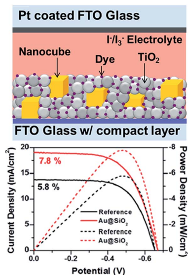
Fig. 15 Schematic illustration of plasmonic DSSC device structure, showing nanocubes embedded within the N719-sensitized mesoporous TiO_2 layer with I^-/I_3^- liquid electrolyte (d) device performance: current density (solid lines) and power density (dashed lines) curves of the DSSCs with and without (reference) Au@SiO 2 core-shell nanocubes. Figure reproduced with permission from ref. 41.
