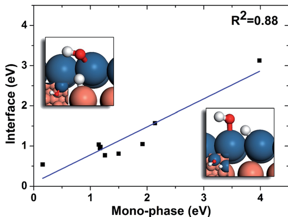
Fig. 6 Linear relation between the barriers of OH hydrogenation on mono-phases and those of interface hydrogens. The geometries of mono-phase hydrogenation of OH and OH hydrogenation on PtCu interface are shown on lower right and upper left, respectively. The blue, brown, white and red balls stand for Pt, Cu, H and O, respectively.
