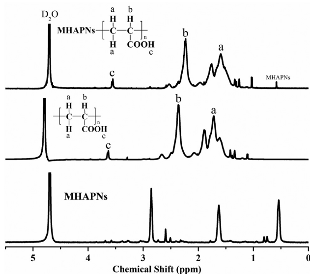
Fig. 3 ^1\text{H} -NMR spectra of the MHAPNs, PAA and PAA-MHAPNs.
