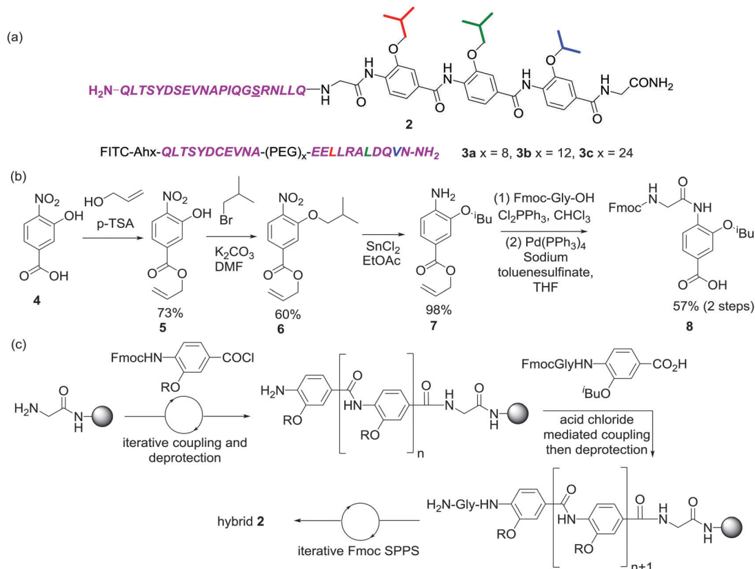
Scheme 1 (a) Structure of peptide-helix mimetic hybrid 2 and 3a–3c (PEG = polyethylene glycol), (b) synthetic route for assembly of the key N-terminal Fmoc glycylyl 3-butyloxy-4-aminobenzoic acid building block 8 (c) outline of approach used to synthesise hybrid 2 .
