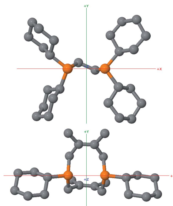
Fig. 8 Ball and stick models of dcpe (top) and \text{Cy}_2\text{-DPC} (bottom) with hydrogen atoms omitted for clarity, highlighting the differences in steric profiles between these two diphosphines. Both ligands are viewed along the Z axis, defined using SambVca 2.0 as the P–Ni–P angle bisector in their respective nickelalactone complexes.
