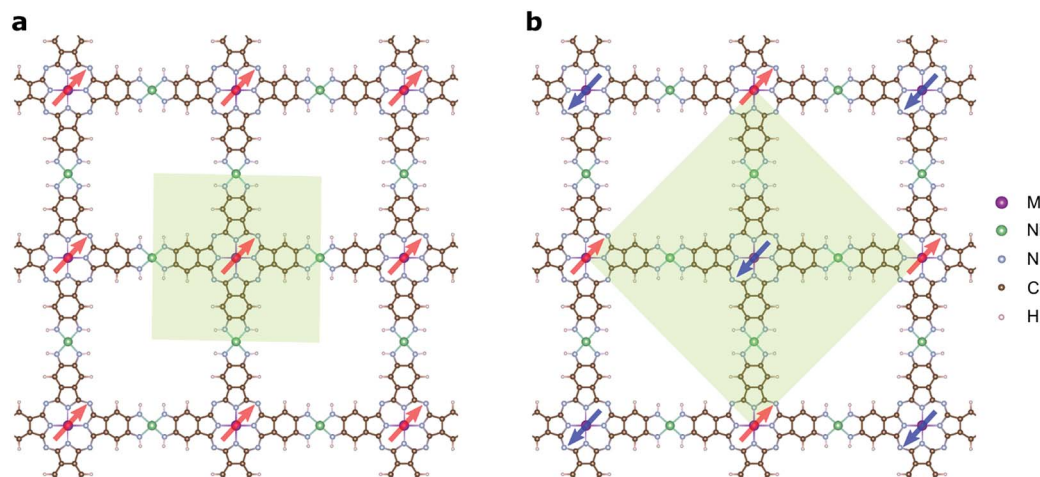
Fig. 3 Magnetic ground states of NiMPC 2D MOFs. Red and blue arrows denote spin-up and spin-down local magnetic moments, respectively. (a) and (b) Illustrate ferromagnetic (FM) and antiferromagnetic (AFM) coupling between metal ions in MPC moieties. The shaded regions in (a) and (b) indicate the structural unit cell and the (\sqrt{2} \times \sqrt{2}) supercell, each corresponding to the magnetic unit cell of the FM and the AFM ground states, respectively.
