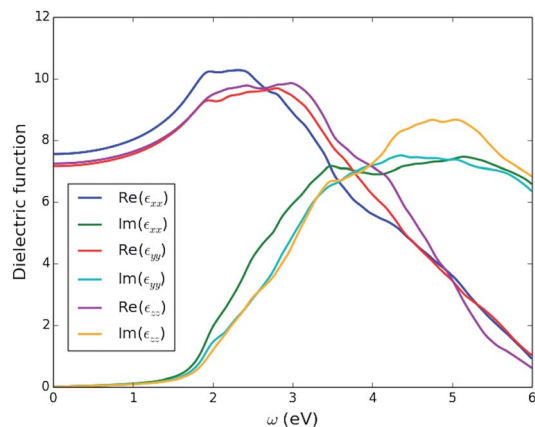
Fig. 13 Three components of the calculated dielectric function, \epsilon(\omega) , as a function of incident photon energy, \omega , for bournonite ( \text{CuPbSbS}_3 ).
