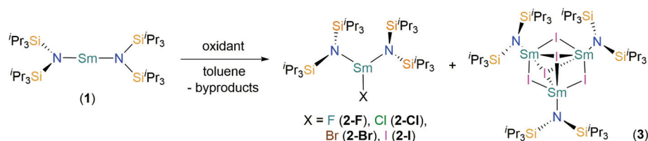
Scheme 1 Synthesis of [Sm(N †† ) 2 (X)] (X = F, 2-F; Cl, 2-Cl; Br, 2-Br; I, 2-I) and [(Sm(N †† )) 3 (μ 2 -I) 3 (μ 3 -I) 2 ] (3) by the treatment of [Sm(N †† ) 2 ] (1) with various oxidants; 2-F: +[Fe(Cp) 2 ][PF 6 ], -[Fe(Cp) 2 ], and PF 5 ; 2-Cl, 2-Br: + t BuX, -CH 3 CH(CH 3 )CH 3 , and -CH 2 =C(CH 3 )CH 3 ; 2-I, 3: +0.5 I 2 and -unidentified by-products.
