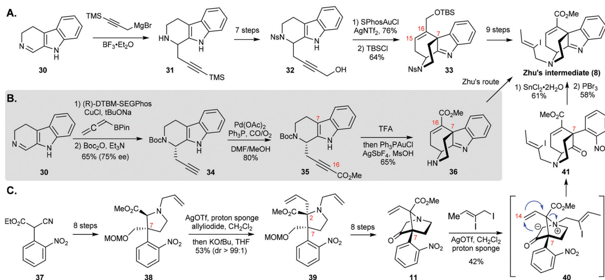
Scheme 6 (A) Ohno's formal synthesis of ( \pm )-strictamine. (B) Snyder's formal synthesis of (+)-strictamine. (C) Gaich's formal synthesis of ( \pm )-strictamine.
