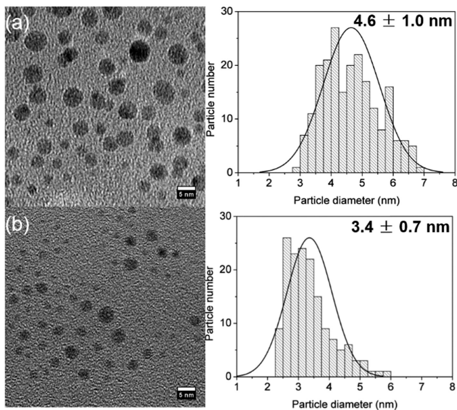
Fig. 5 Size and size distribution Ag nanoparticles from (a) SHR and (b) CFIR; helix diameter: 10 mm, pitch distance: 1/\pi cm, length: 1 m, 0.03" ID. 0.6 mM NaBH 4 , 0.1 mM AgNO 3 , total flow rate: 0.7 ml min -1 , 60 °C, residence time: 39 s.
