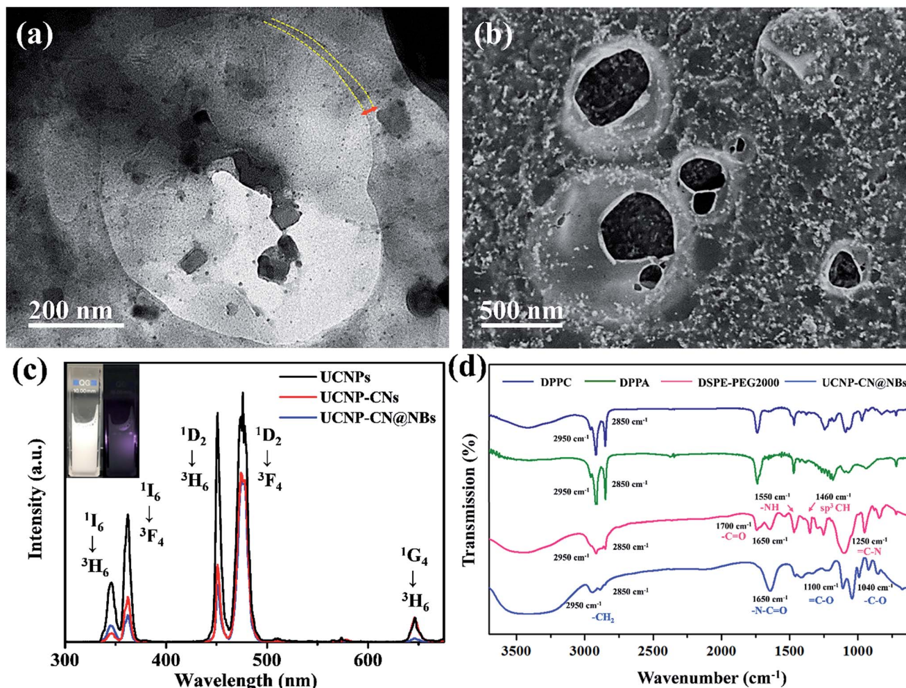
Fig. 3 (a) TEM and (b) SEM images of UCNP-CN@NBs. (c) UV-vis and photoluminescence spectra of UCNP-CN@NBs. UCNP-CN@NBs were irradiated by a 808 nm laser at 0.5 \text{ W cm}^{-2} . (d) FTIR spectra of UCNP-CN@NBs.
