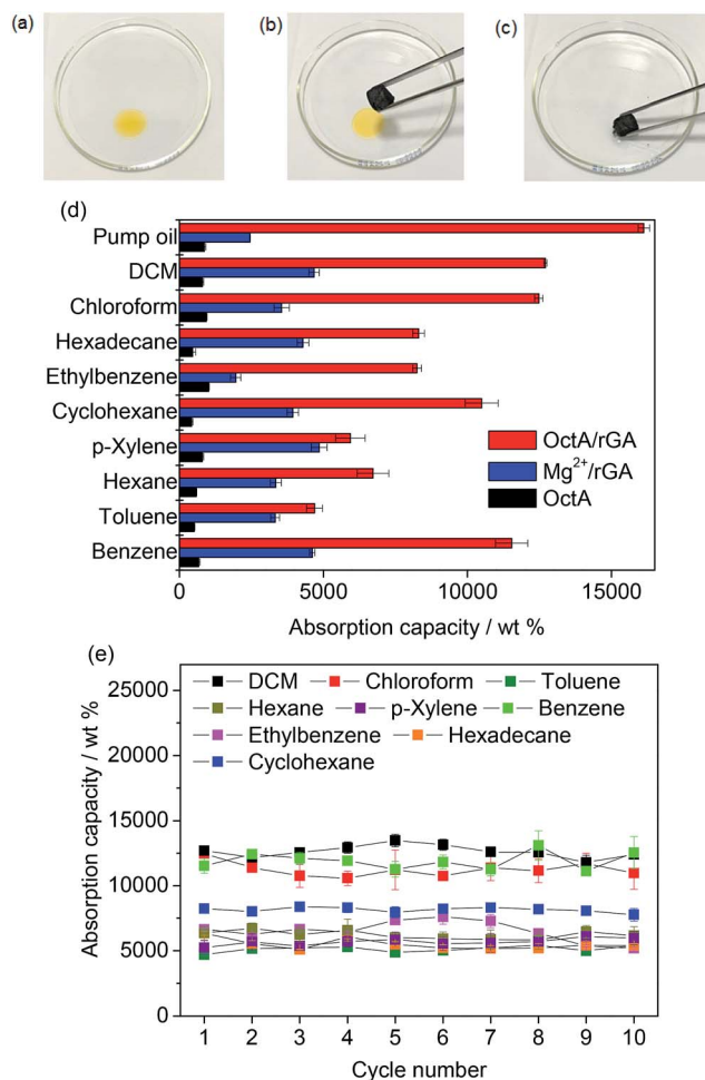
Fig. 4 Absorption process of hexadecane colored with Sudan I by OctA/rGA: (a and b) before absorption and (c) after absorption. (d) Absorption capacities of OctA/rGA with various organic liquids. (e) Recyclability tests of absorption capacities of OctA/rGA for organic liquids.
