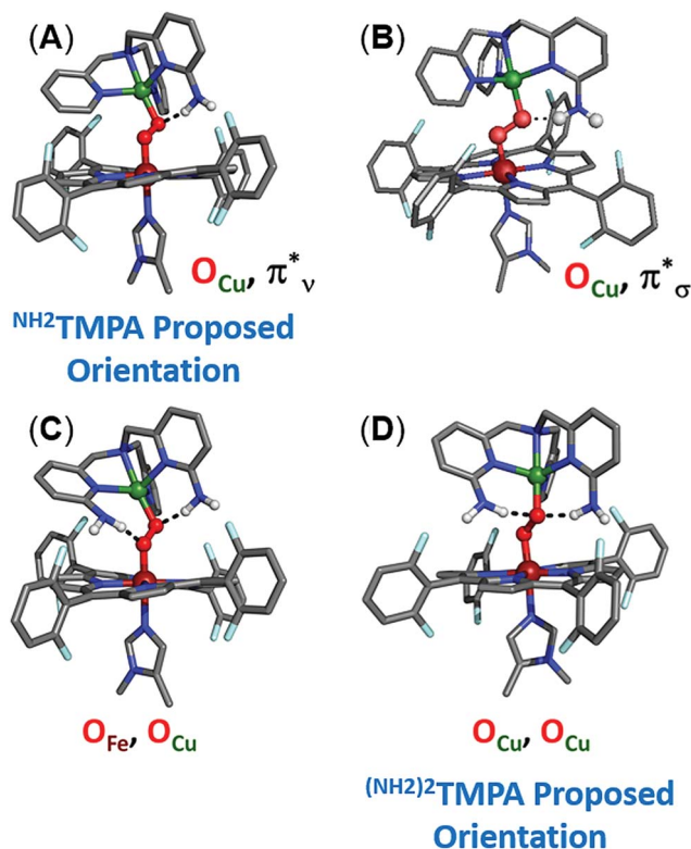
Fig. 10 Optimized DFT structures of \text{LS}^{\text{-NH}_2}\text{TMPA} (top: (A) and (B)) and \text{LS}^{(\text{NH}_2)_2}\text{TMPA} (bottom: (C) and (D)) indicating which orientation of the \text{-NH}_2 moieties is preferred in H-bonding to the peroxy core.
