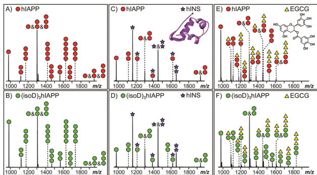
Fig. 1 The MS spectra of the 10 \mu\text{M} solutions hIAPP (A; red circle) and (isoD) 3 hIAPP (B; green circle) only, the 10 \mu\text{M} solutions of (C) hIAPP and (D) (isoD) 3 hIAPP mixed with 10 \mu\text{M} hINS (purple star); the 10 \mu\text{M} solutions of (E) hIAPP and (F) (isoD) 3 hIAPP mixed with 10 \mu\text{M} EGCG (yellow triangle).
