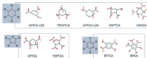
Fig. 6 The orientation of the COOH along the cyclic 6-membered ring, 5-membered ring and benzene ring. TPCHTCA (DEVKOW); 24 THFTCA (ZEZLEV); 25 BTTCa (PYMELL12); 26 BHCA (MELLIT). 27
