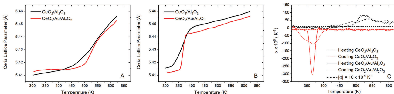
Fig. 3 Experimental DXP results showing the extracted ceria lattice parameter. The ceria/alumina and ceria/Au/alumina ceria lattice parameter refinements are given in black and red respectively for experiments conducted during heating in a 5% H 2 /He atmosphere for the ceria (A) and cooling (B) in 5% H 2 /He (C) instantaneous expansion coefficient during heating and cooling for the ceria/alumina (dotted lines) and ceria/Au/alumina (solid lines) samples. Dashed lines give the expected thermal expansion coefficient of ceria, \alpha = 10 \times 10^{-6} \text{ K}^{-1} , expansion in excess is associated to chemical change of the sample.
