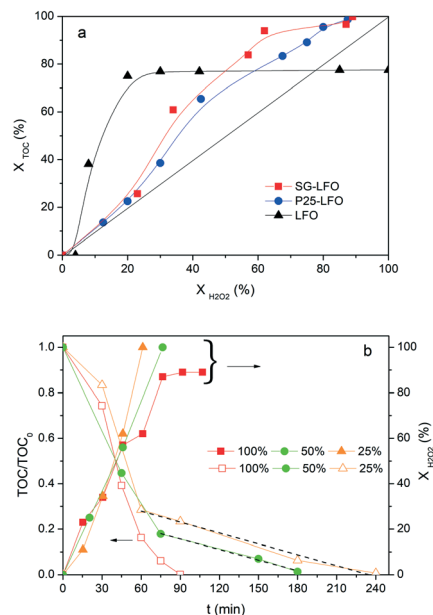
Fig. 7 a) TOC conversion vs. H_2O_2 conversion for the combined photo-Fenton and photocatalytic degradation of 4-CP over the pristine and the Ti-substituted LaFeO_3 catalysts. Conditions: [4-CP]_0 = 25 \text{ mg L}^{-1} ; [H_2O_2]_0 = 125 \text{ mg L}^{-1} ; T = 25 \text{ }^\circ\text{C} ; [cat] = 0.5 \text{ g L}^{-1} ; UV-A irradiance of 60 \text{ W m}^{-2} . b) Influence of the H_2O_2 dose on the relative TOC concentration time-evolution and the H_2O_2 conversion obtained for the SG-LFO catalyst. Conditions: [4-CP]_0 = 25 \text{ mg L}^{-1} ; [H_2O_2]_0 = 31.25\text{--}125.00 \text{ mg L}^{-1} , corresponding to the 25–100% range; T = 25 \text{ }^\circ\text{C} ; [cat] = 0.5 \text{ g L}^{-1} ; UV-A irradiance of 60 \text{ W m}^{-2} . Taking into account that the experiments were carried out using the stoichiometric amount of H_2O_2 to mineralize TOC, the linear curve with a unity slope reflects the implementation of a heterogenized photo-Fenton process with no occurrence of scavenging reactions.
