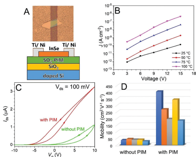
Fig. 4 (A) Schematic of the InSe-based FET device and the top-view optical microscopy image. (B) Leakage current density as a function of voltage in a capacitor device. (C) The I_{ds}-V_g transfer curve and (D) comparison of electron mobility in InSe for the FET devices with and without SO 2 -PIM. Five devices were tested for each type of FET.
