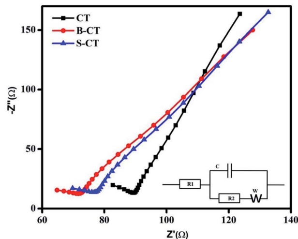
Fig. 5 Nyquist plots of CT, S-CT and B-CT.
