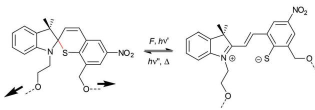
Scheme 35 Mechanochemical isomerization of spirothiopyran to thiomercyanine.
