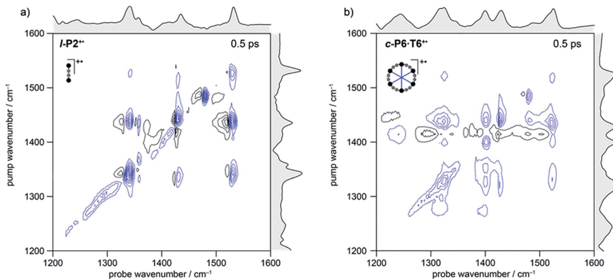
Fig. 3 2D-IR spectra of l -P2 + (a) and c -P6·T6 + (b) at 500 fs delay in the fingerprint region. Black solid and blue dashed contour lines correspond to positive (ESA) and negative (GSB) signals, respectively. Contours near zero are hidden for clarity. Spectra were recorded using a broadband pump centered at \sim 1325 \text{cm}^{-1} (FWHM \sim 150 \text{cm}^{-1} ). Optical densities of all samples were \sim 0.2 – 0.4 in the fingerprint region. Linear FTIR spectra are shown in gray along each axis.
