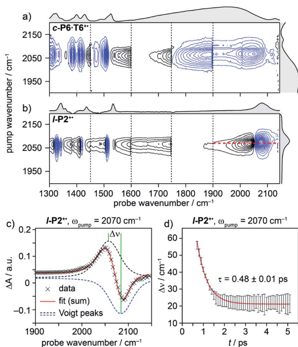
Fig. 4 2D-IR spectra of c -P6·T6 + (a) and l -P2 + (b) at 400 fs delay, with pump (FWHM \sim 80 \text{cm}^{-1} ) centered at 2080 \text{cm}^{-1} . Black solid and blue dashed contour lines correspond to positive (ESA) and negative (GSB) signals, respectively. Vertical dashed lines correspond to different experimental spectra, where probe a was changed to cover region 1300 – 1900 \text{cm}^{-1} and probe b was centered in the 1900 – 2150 \text{cm}^{-1} region for each experiment (see Fig. S14–S23 † for time resolution of each probe window). Probe windows in 1300 – 1900 \text{cm}^{-1} were stitched together by normalizing all probe a spectra to probe b . (c) fit of on-diagonal slice for l -P2 + (red line in (b)) using the sum of two Voigt. (d) The peak–peak distance for each time delay, calculated from the fit in (c).
